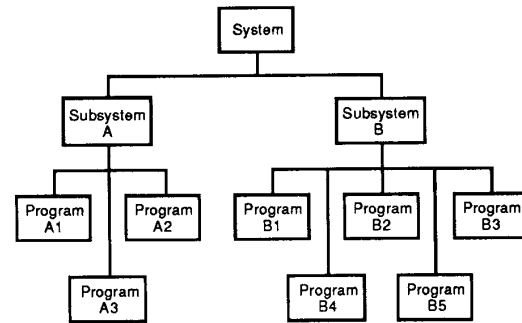
Fig 16 Structure Chart
