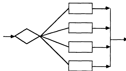
Fig 5 Case Construct
